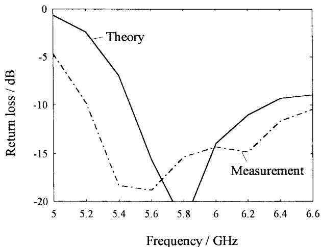
Fig. 4. Output return loss of active antenna.
