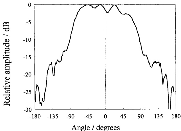
Fig. 6. E -plane radiation diagram of the active antenna ( f = 5.8 GHz).
