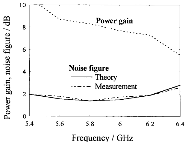
Fig. 5. Experimental power gain (compared to a passive antenna) and noise figure of the active antenna.
